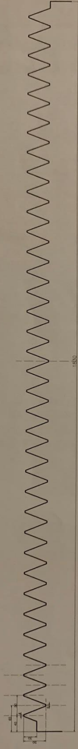
DETAIL FOR DELIVERY ROLLER (No of teeth 36)
